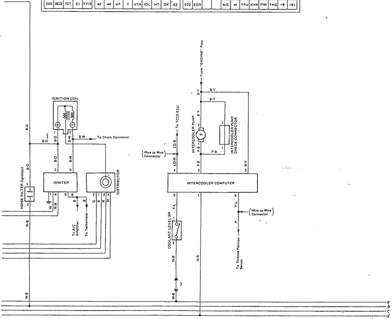
Toyota Computer Control System Wiring Circuit (Part 2 Of 2). Celica w/3S-GTE Engine
