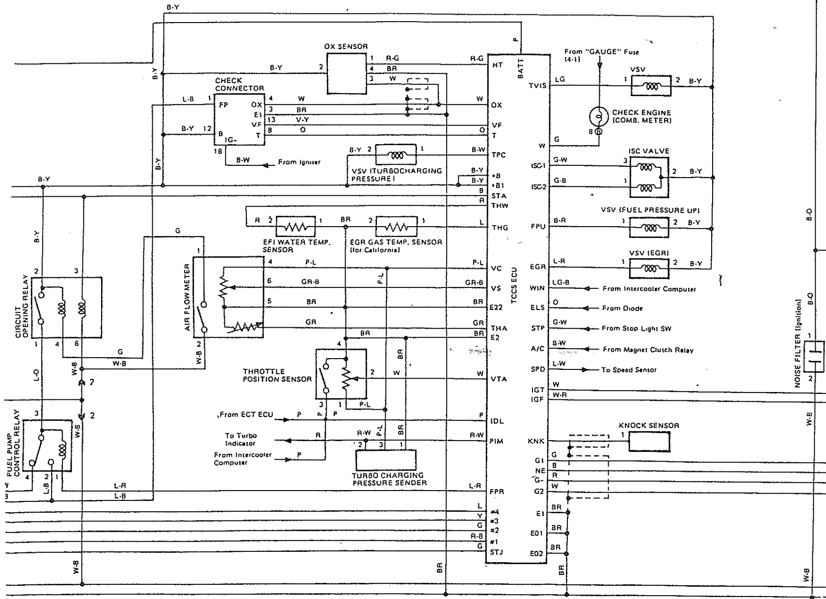
Toyota Computer Control System Wiring Circuit (Part 1 Of 2). Celica w/3S-GTE Engine
